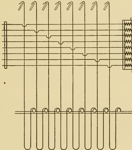
Fig. 1. Common Jacquard Hook.
